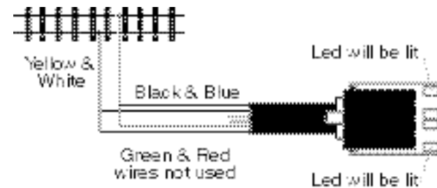
LT-1 Set Up As A Track Tester
