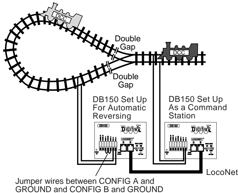
Diagram 4: Automatic Reversing Section
