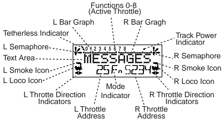
Diagram 7: DT300 LCD
