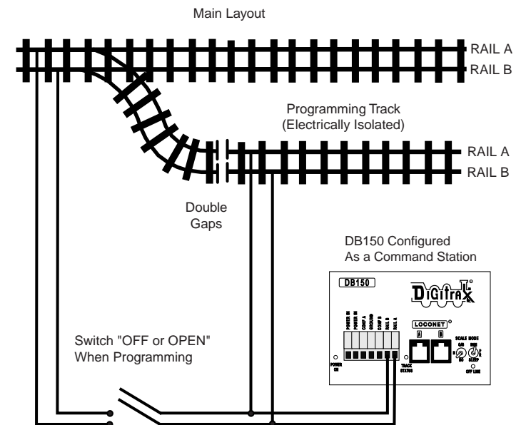
Diagram 3: Programming Track
