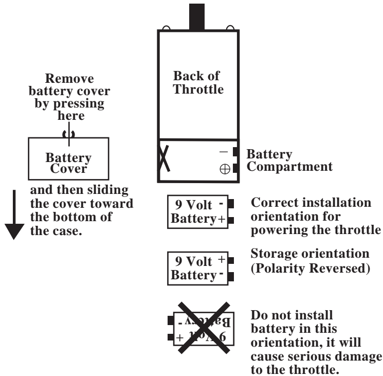
Diagram 8: DT300 Battery Installation
